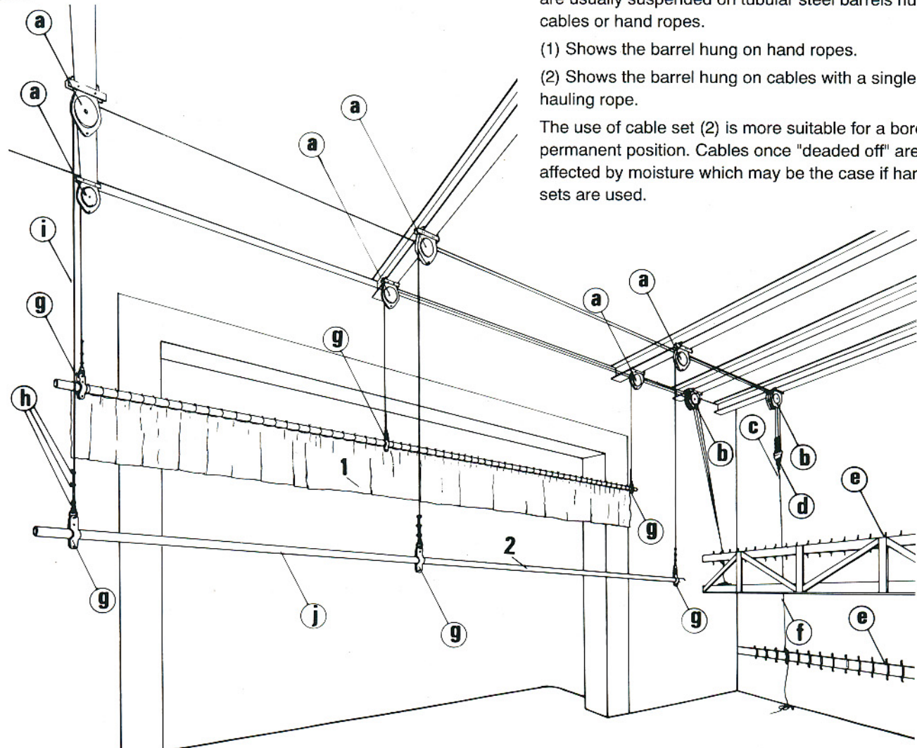
Alternative cable connection to barrel giving simple level adjustments.
